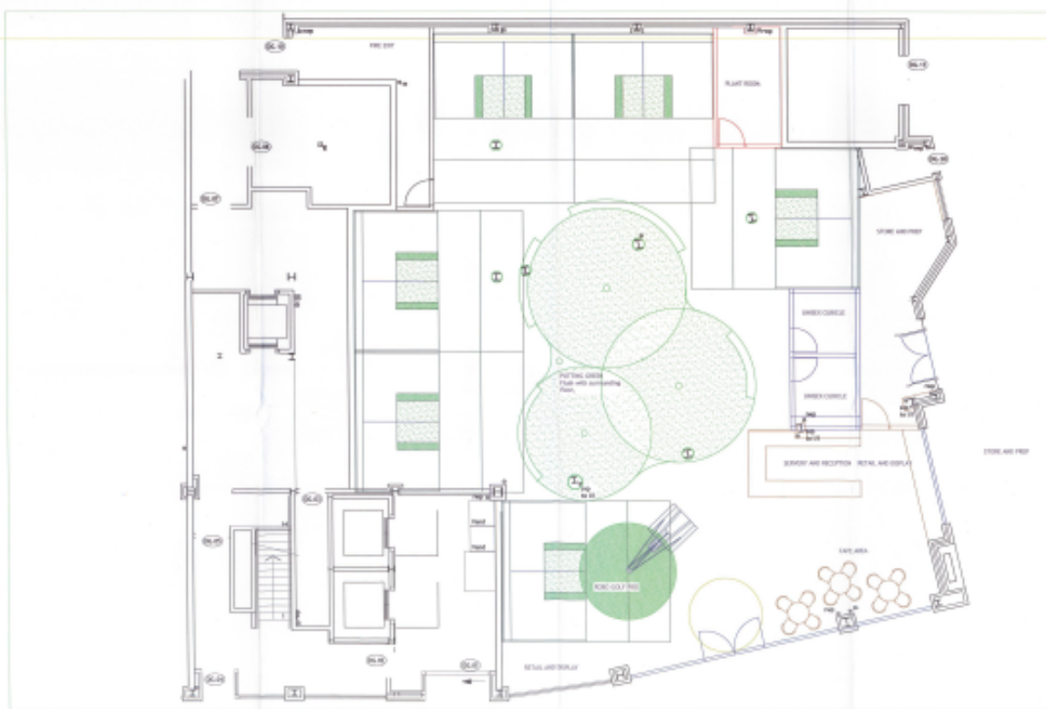
Proposed Layout
